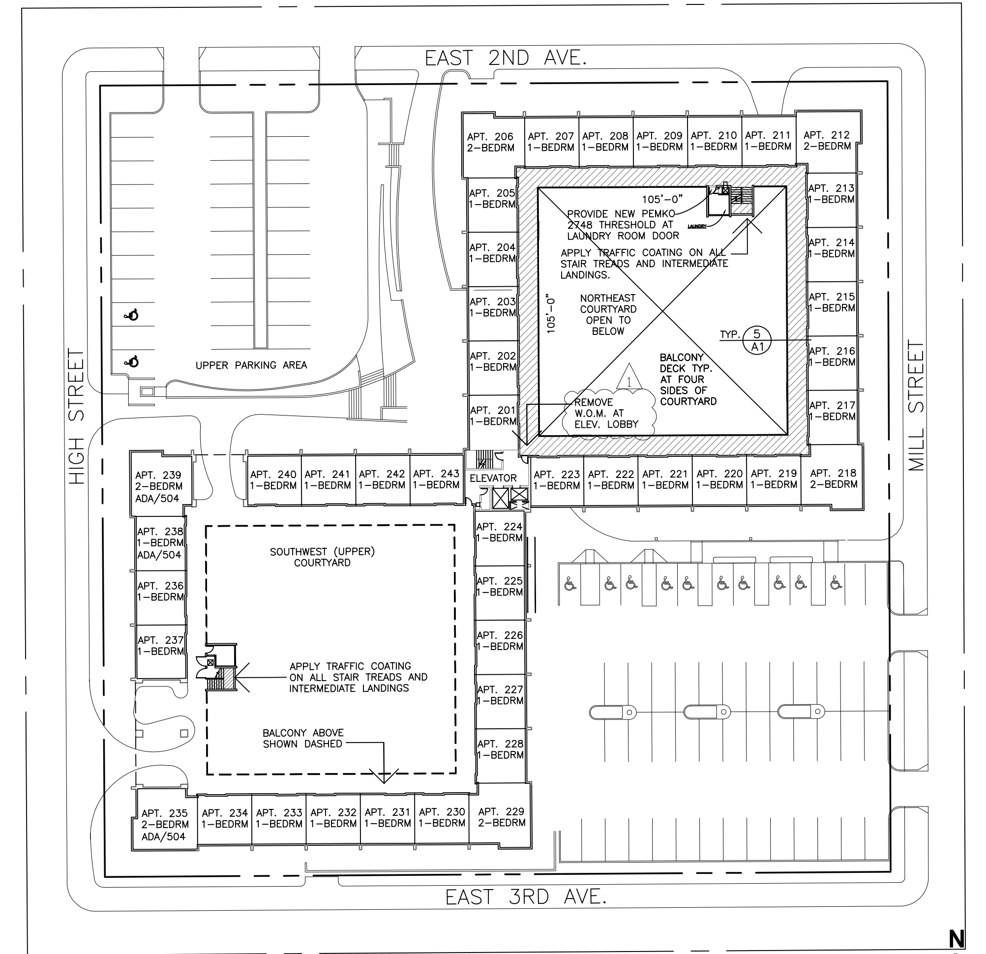
2 A1 SECOND FLOOR PLAN 1" = 40'-0"
