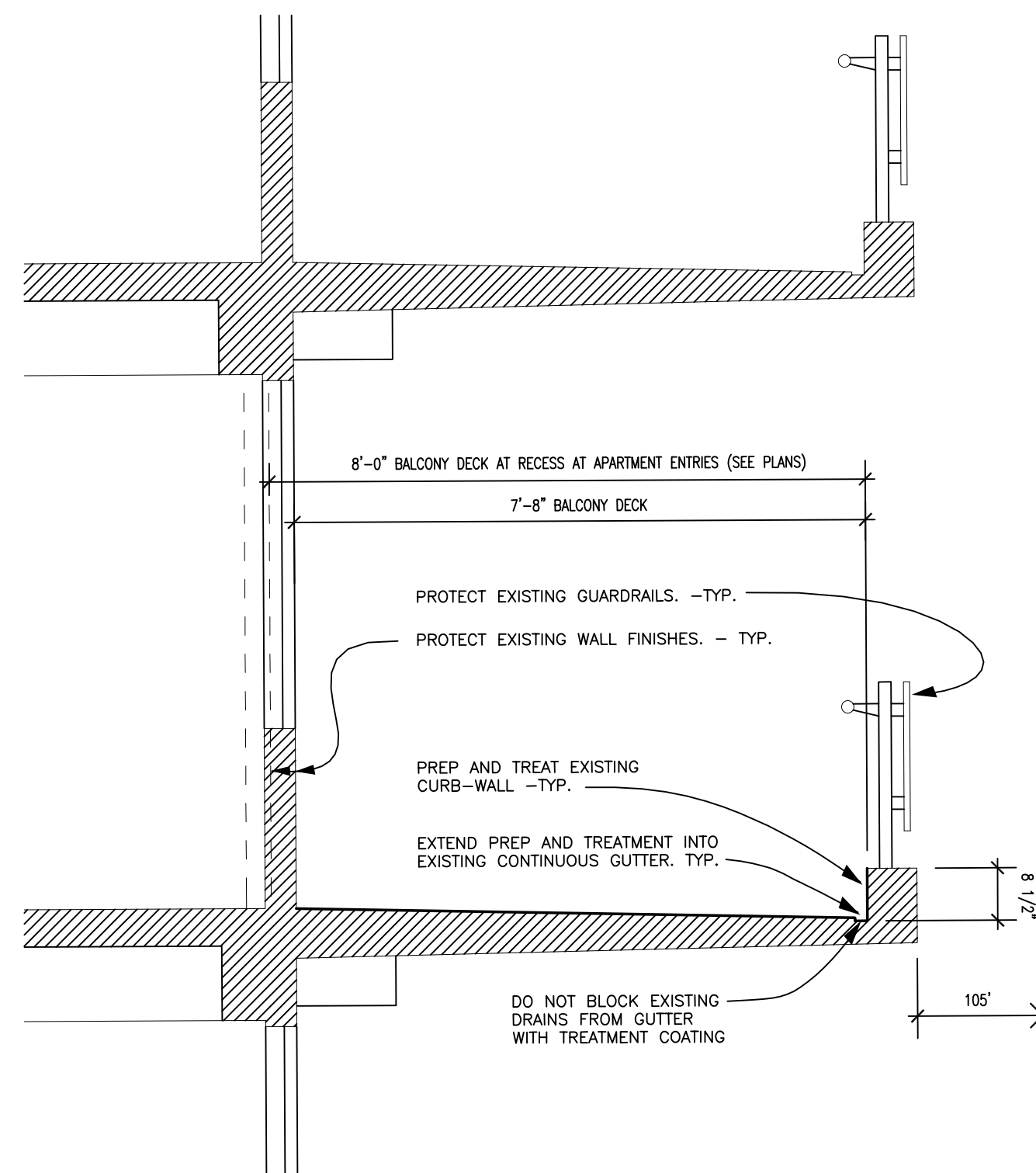
5 A1 SECTION THROUGH BALCONY 1/2" = 1'-0"
